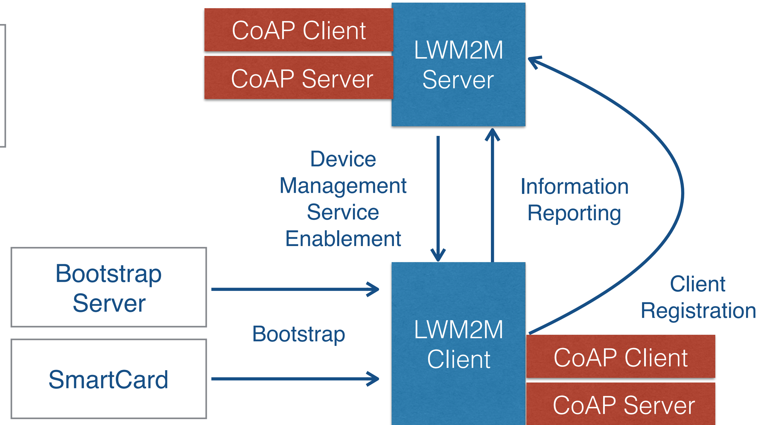
LWM2M Architecture
